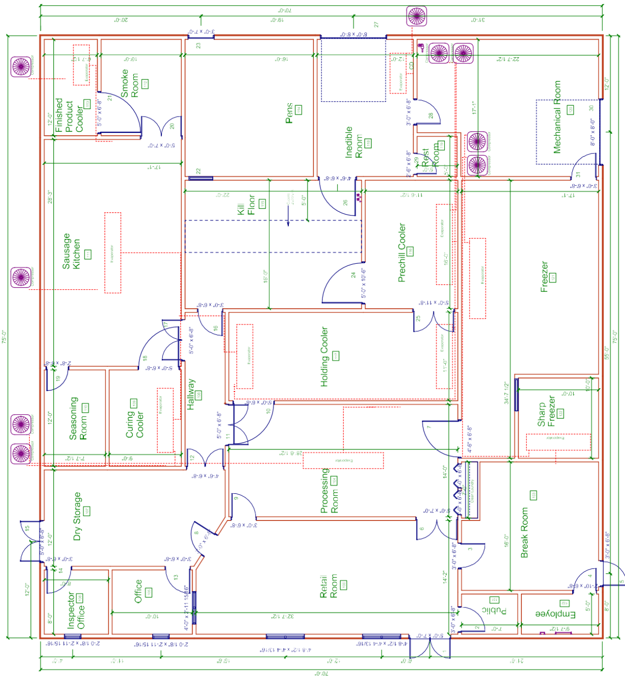
Refrigeration Plan
