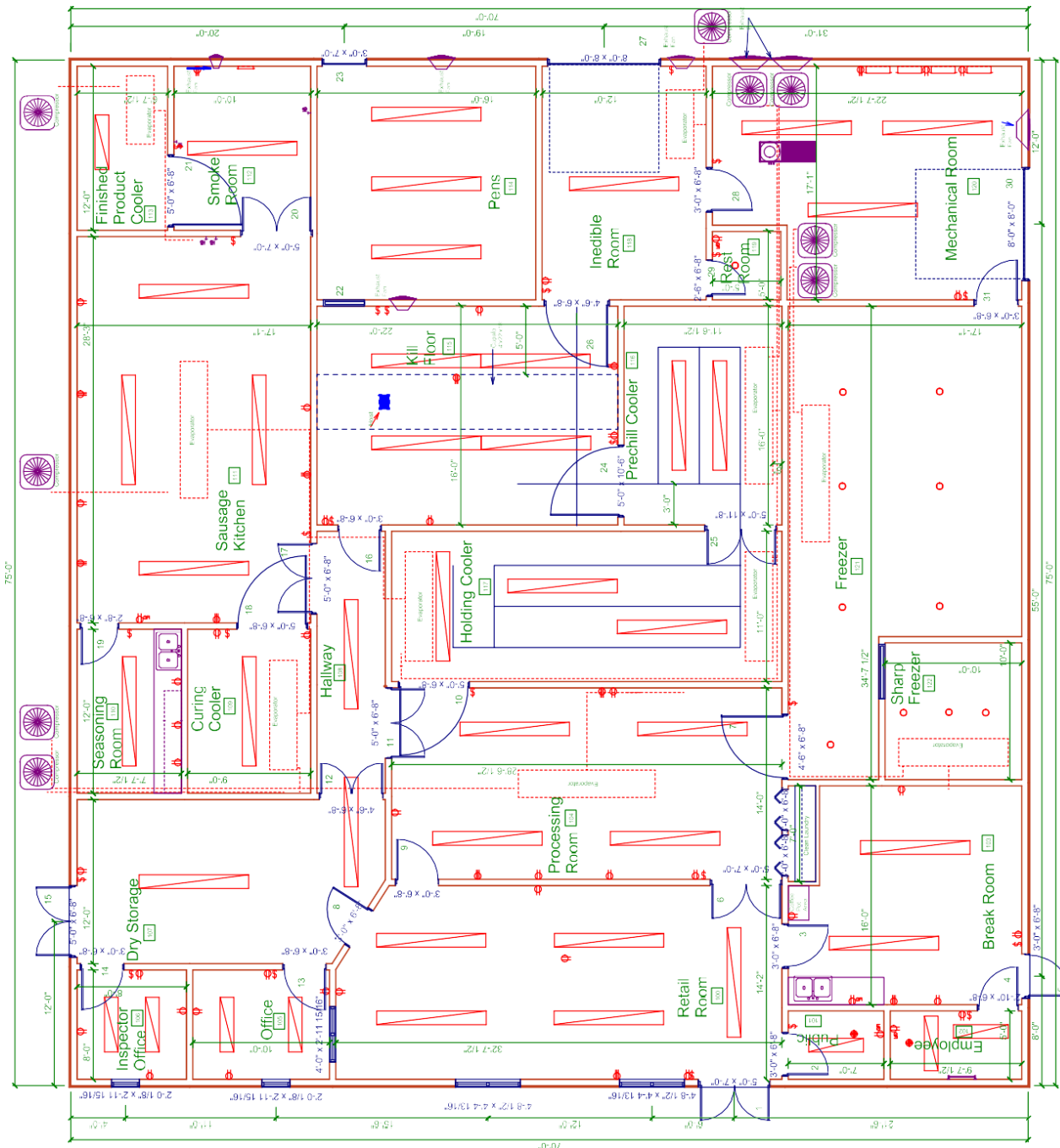
Electrical Plan
